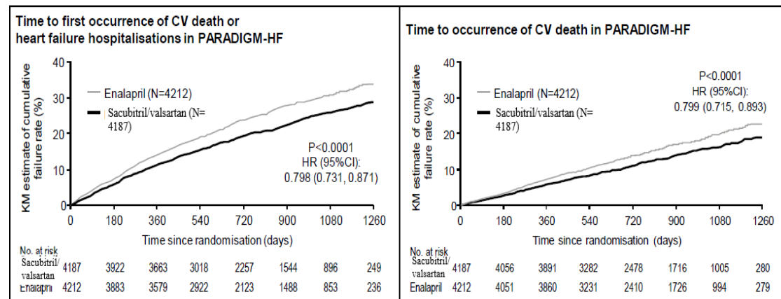
Figure 1 Kaplan-Meier curves for the primary composite endpoint and the CV death component
