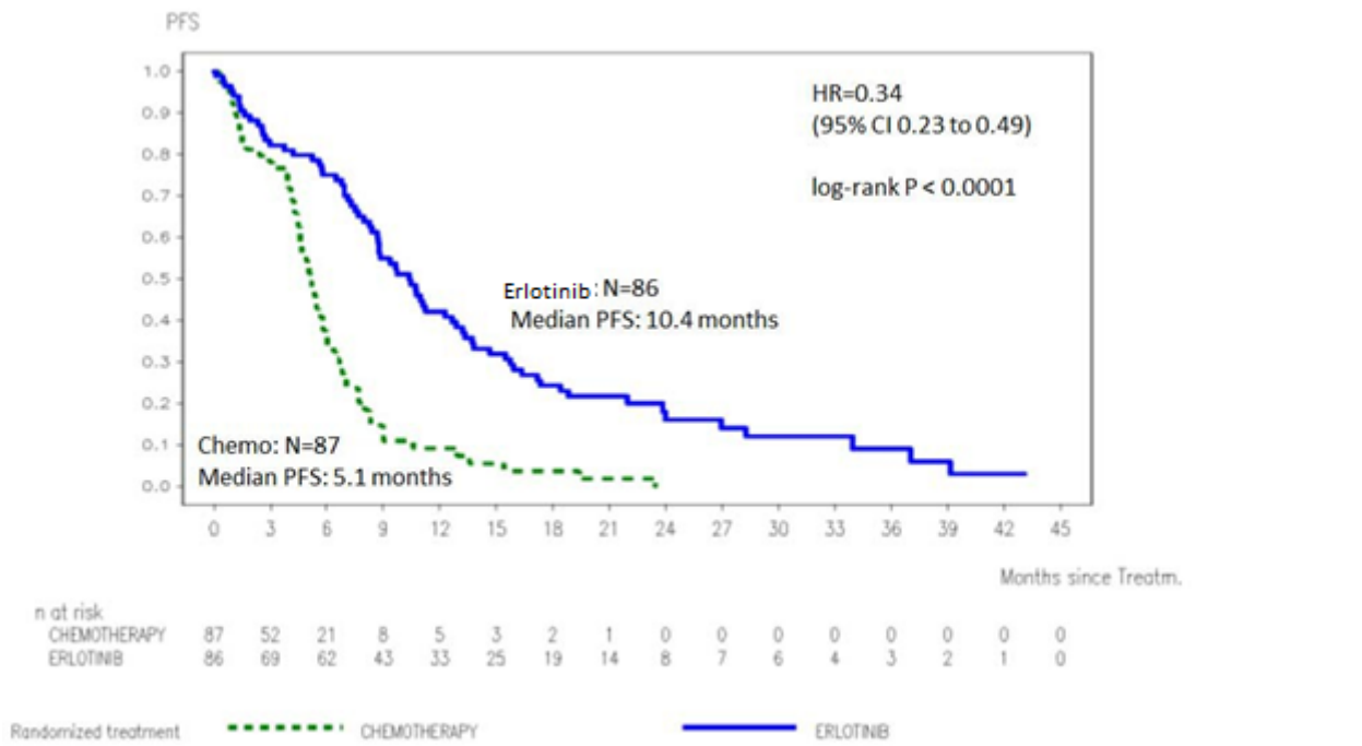
Figure 1: Kaplan-Meier curve for investigator assessed PFS in trial ML20650 (EURTAC) (April 2012 cut-off)
