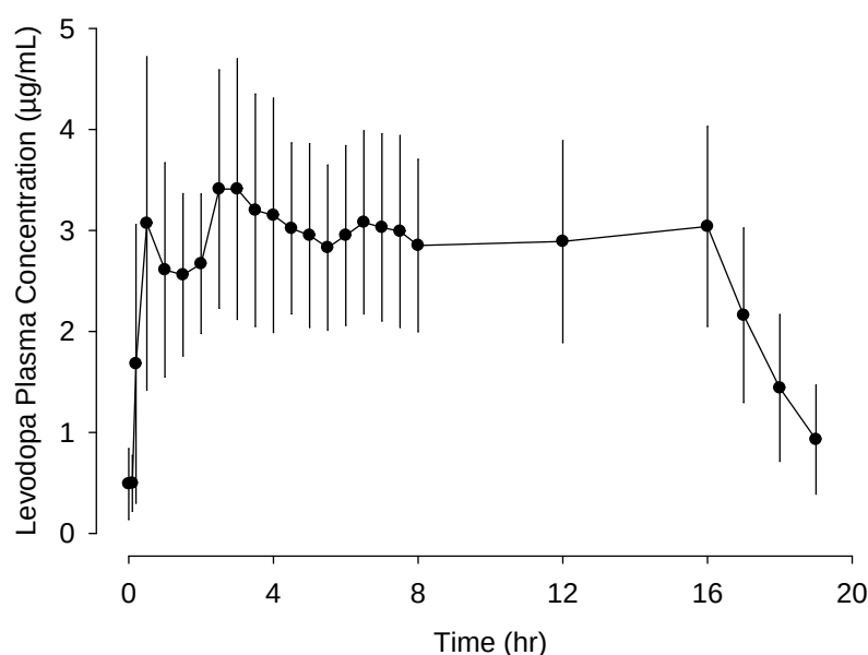
Figure 1. Plasma Concentrations (mean \pm standard deviation) versus Time Profile of Levodopa with Duodopa 16-Hour Infusion
